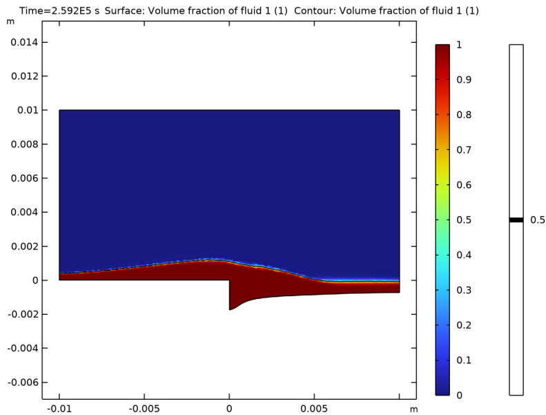
Figure 2: The corrosion product deposition and dissolution of magnesium after 72 h.
