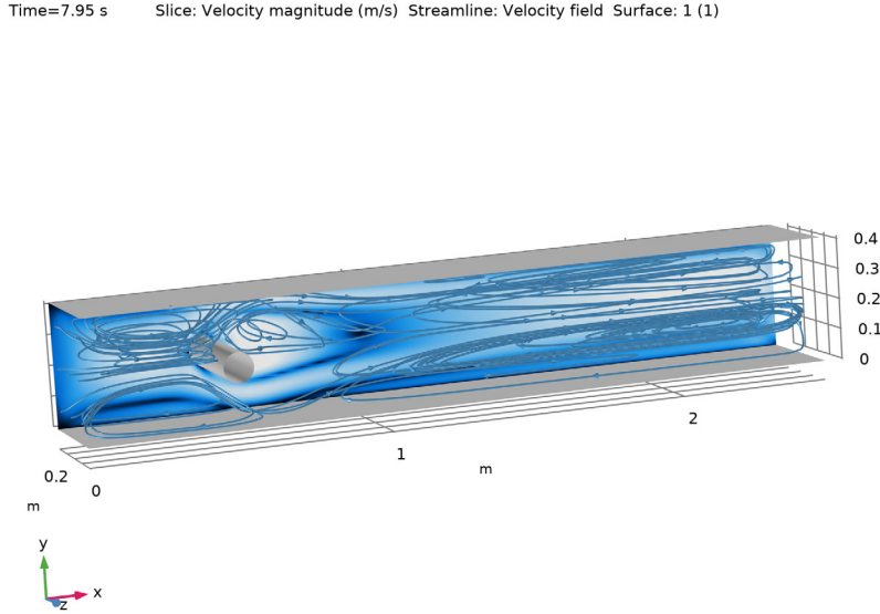
Figure 3: Computed velocity field at t = 7.95 s.
