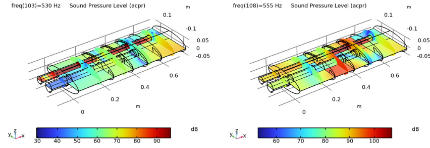
Figure 8: Sound pressure level distributions at 530 Hz (left) and 555 Hz (right).
