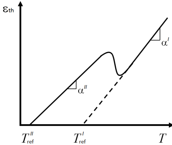
Figure 3-5: Thermal strain during phase transformation.
