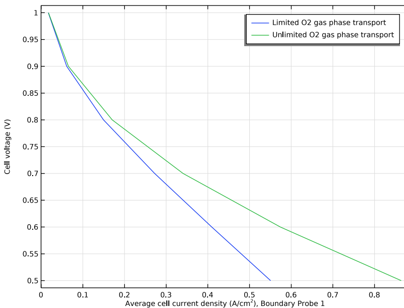
Figure 6: Polarization plot.
