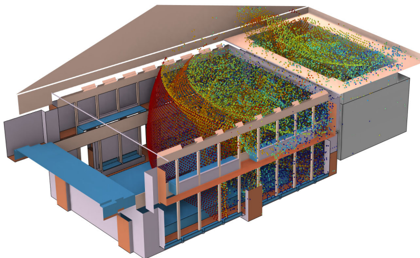
Figure 8: Ray tracing model of a chamber music hall including the ray location at 35 ms. Figure taken from the Chamber Music Hall model found in the Application Library.
