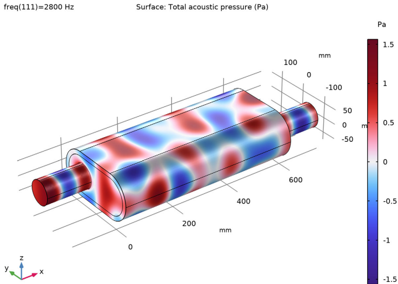
Figure 10: The pressure distribution in the absorptive muffler without the liner is shown for f = 2800 Hz.
