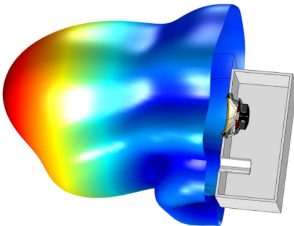
Figure 5: A 3D bubble plot of the loudspeaker radiation patten at 3000 Hz. From the Vented Loudspeaker Enclosure model found in the application library.
