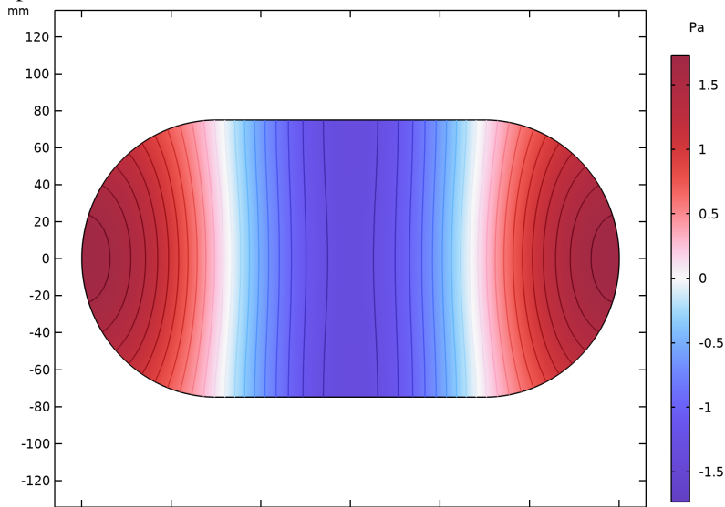
Figure 13: First fully symmetric propagation mode of the muffler chamber (with no absorbing liner). The plot shows the real part of the pressure.
