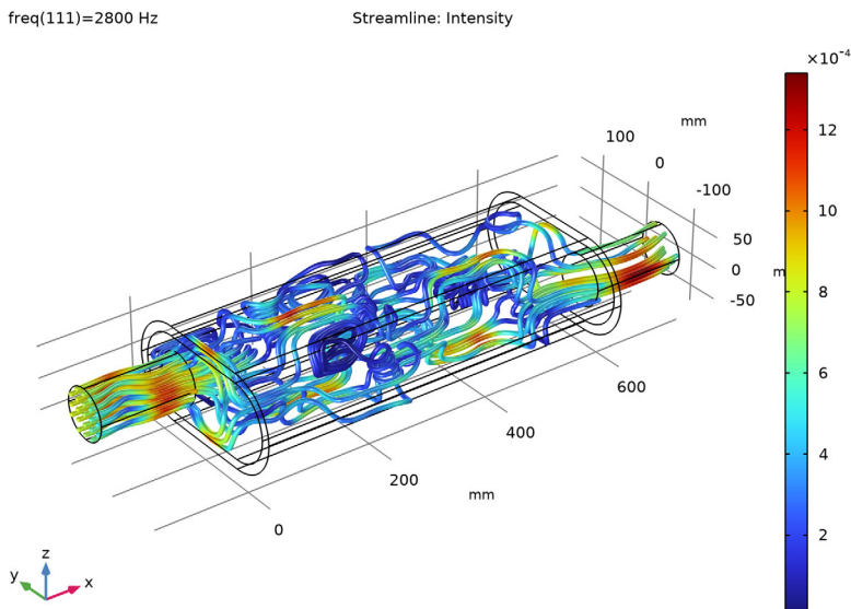
Figure 12: Intensity streamlines at 2800 Hz without the liner.
