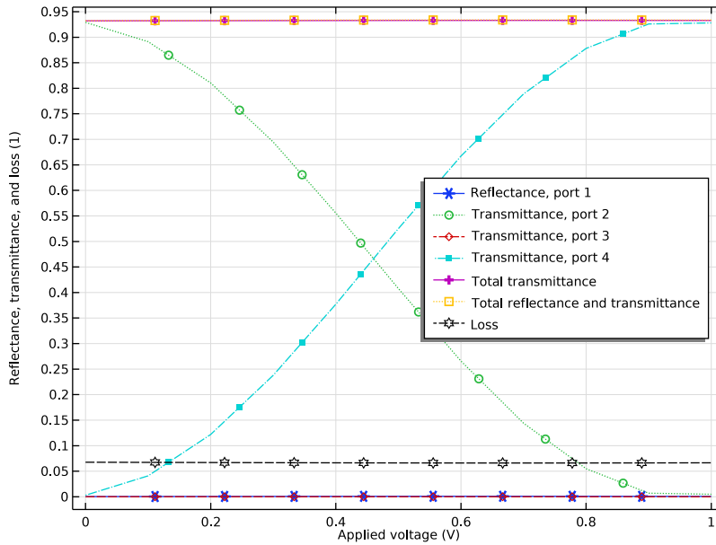
Figure 6: The transmission to the upper (port 2) and the lower (port 4) output waveguide versus the applied voltage, V_0 .
