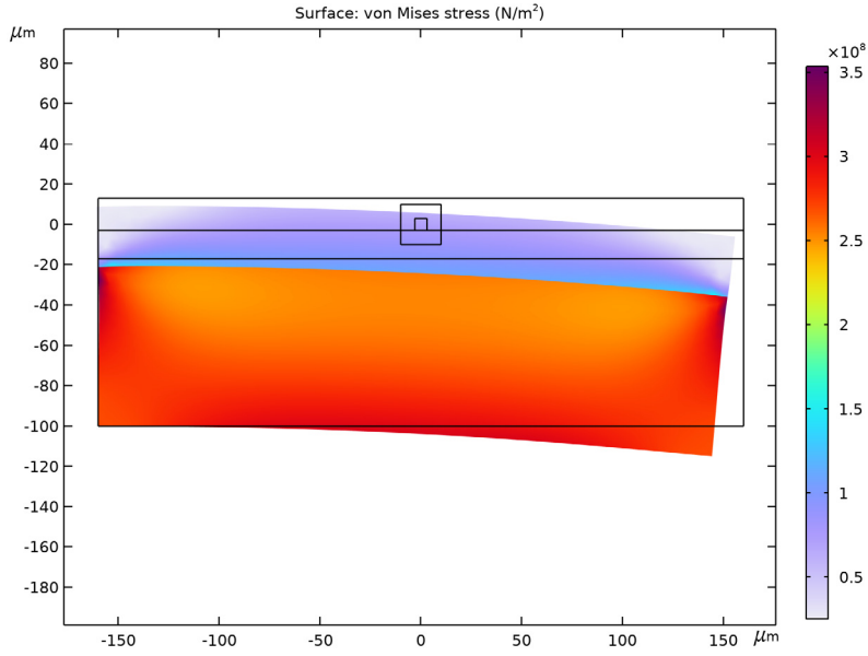
Figure 1: von Mises equivalent stress.
