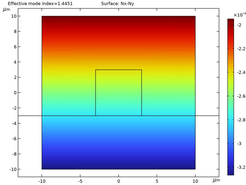
Figure 2: Birefringence.
