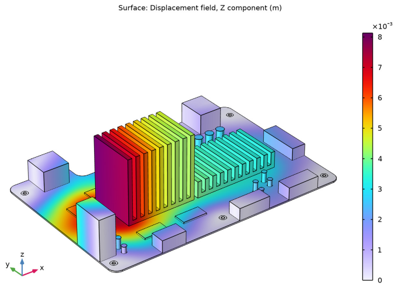
Figure 8: Vertical displacement, as a result of the response spectrum evaluation.
