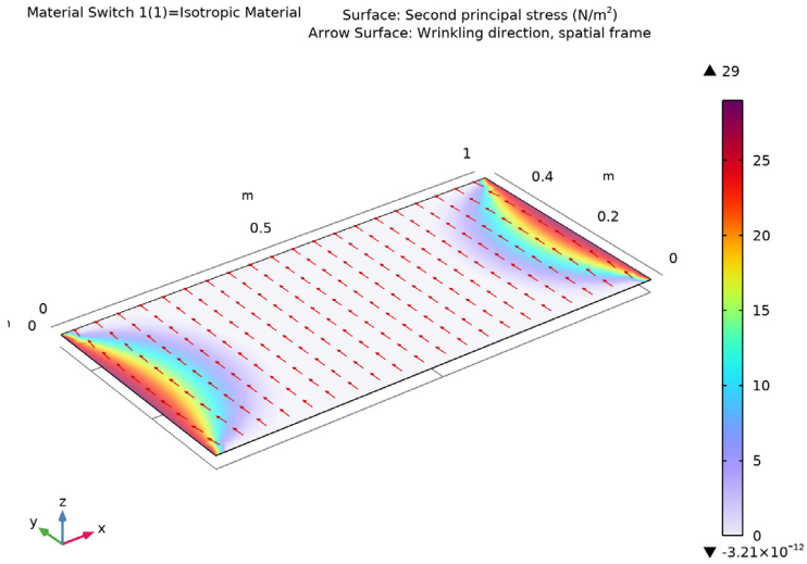
Figure 7: Second principal stress, isotropic material.
