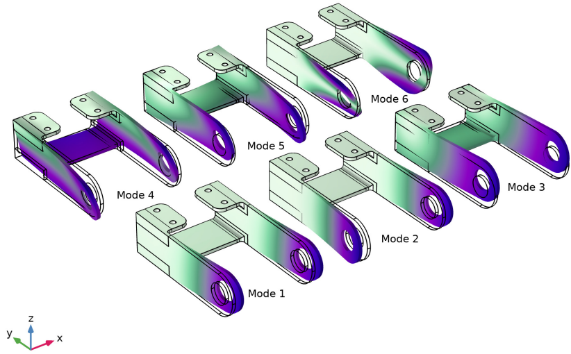
Figure 2: Six first eigenmode shapes for the unloaded case.
