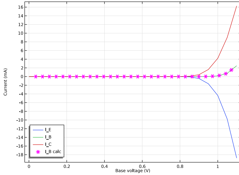
Figure 4: Terminal currents as a function of the base-emitter voltage ( V_{BE} ) for a fixed collector-emitter voltage ( V_{CE} = 0.5 \text{ V} ).
