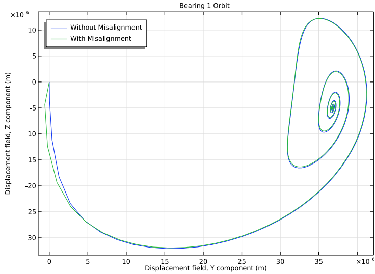
Figure 4: Journal orbit in left bearing.
