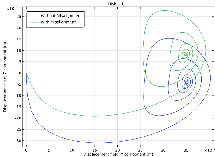
Figure 7: Rotor orbit at disk.
