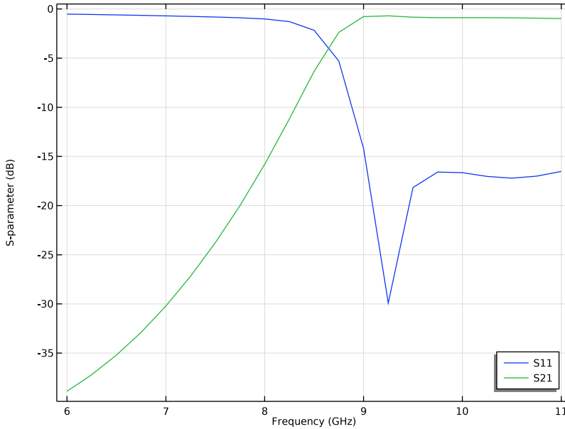
Figure 2: Frequency response of the substrate integrated waveguide resembles that of a conventional rectangular waveguide.
