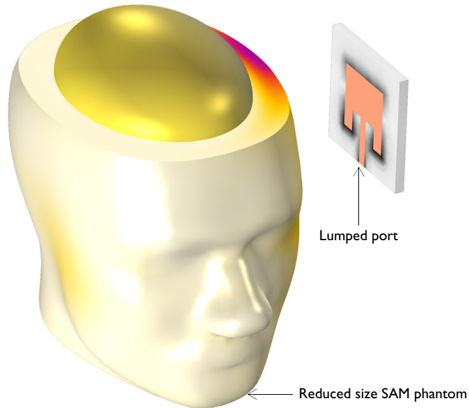
Figure 1: Human head phantom next to a microstrip patch antenna resonant around the Wi-Fi frequency range. The surrounding air domain and perfectly matched layer are removed from the figure for visualization purposes.
