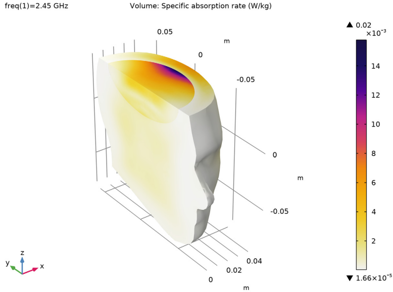
Figure 2: The computed local SAR values are visualized for a part of the head using a filter subfeature. The brain part closest to the radiating antenna has the highest SAR values.
