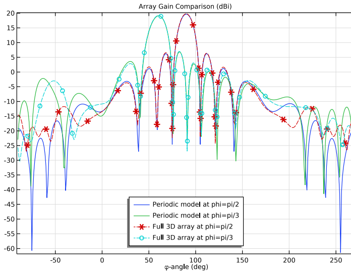
Figure 8: Gain comparison in a 1D plot. 1D plot perspective, different from the polar plot, provides a better view while observing nulls and backlobes.
