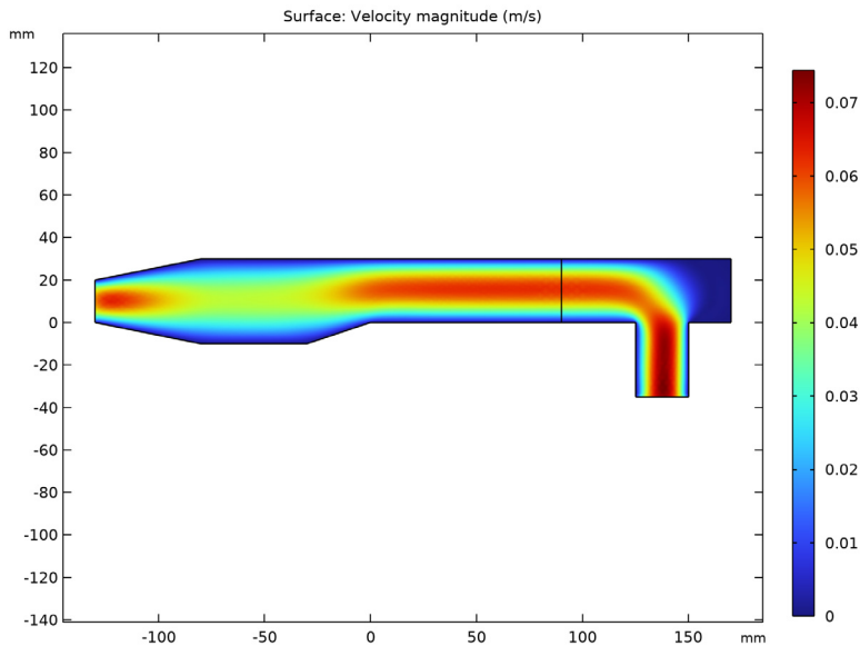
Figure 2: Velocity magnitude.
