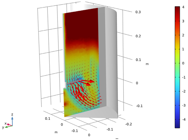
Figure 4: Logarithm of the effective viscosity for N_{\text{Re}} = 400 . Arrows show the velocity field.
