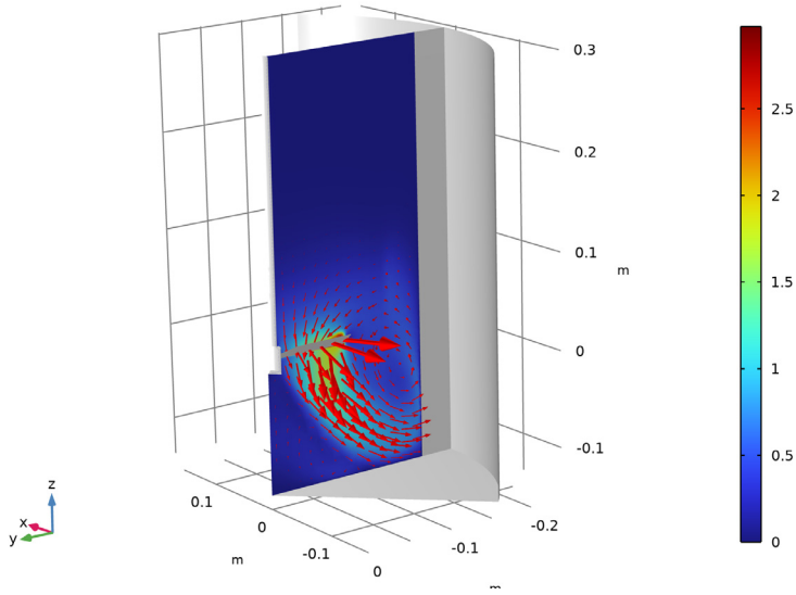
Figure 3: Velocity vectors and velocity magnitude for N_{\text{Re}} = 400 .
