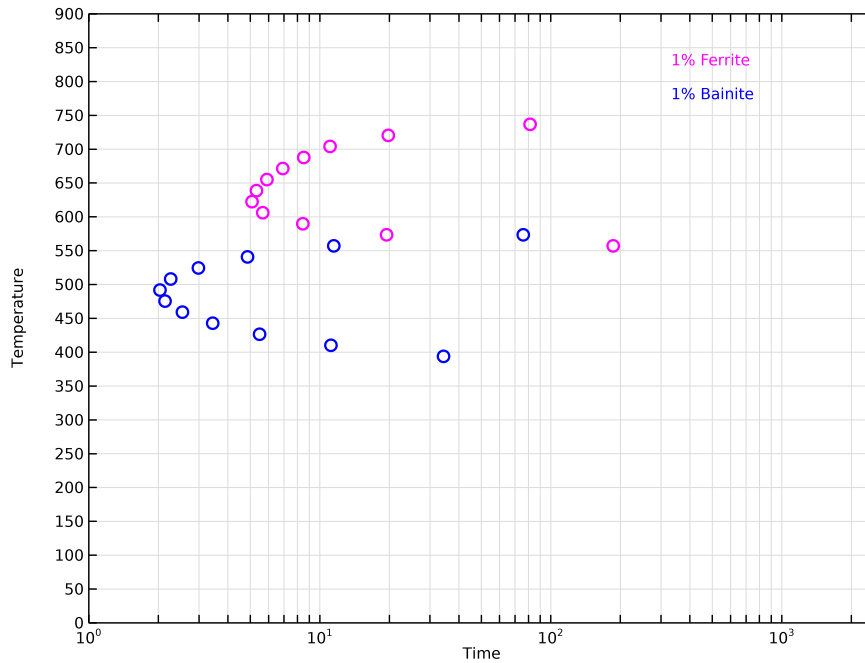
Figure 4: Computed TTT diagram showing the curves for 1% formed fraction of ferrite and bainite.
