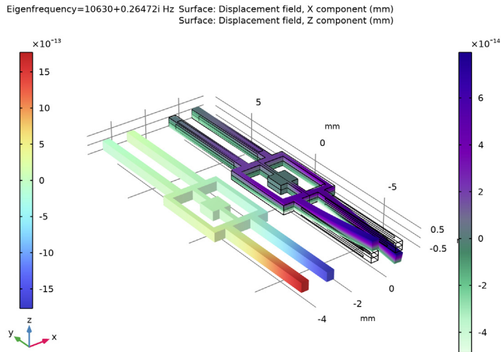
Figure 2: Drive mode, showing both in-plane motion (right) and out-of-plane motion (left). Note that the amplitude scale is arbitrary — only the relative value of the in-plane and out-of-plane displacements has physical significance.
