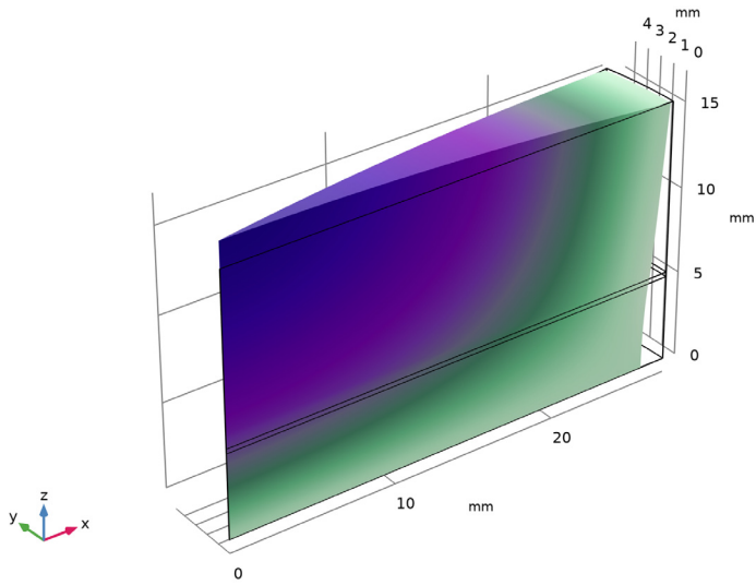
Figure 1: The lowest vibration eigenmode of the transducer.
