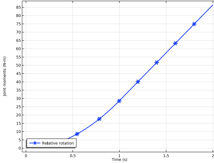
Figure 12: Relative rotation of the arms at the hinge joint (Case-5).
