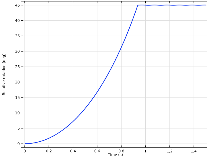
Figure 7: Relative rotation of the arms at the hinge joint (Case-3).
