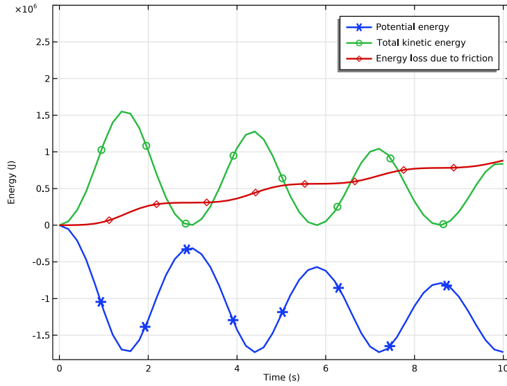
Figure 15: Time variation of different forms of energy (Case-6).
