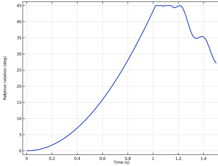
Figure 4: Relative rotation of the arms at the hinge joint (Case-2).
