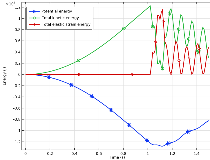
Figure 6: Time variation of different forms of energy in Case-2.
