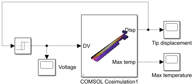
Figure 1: Simulink diagram of the thermal actuator controller.
