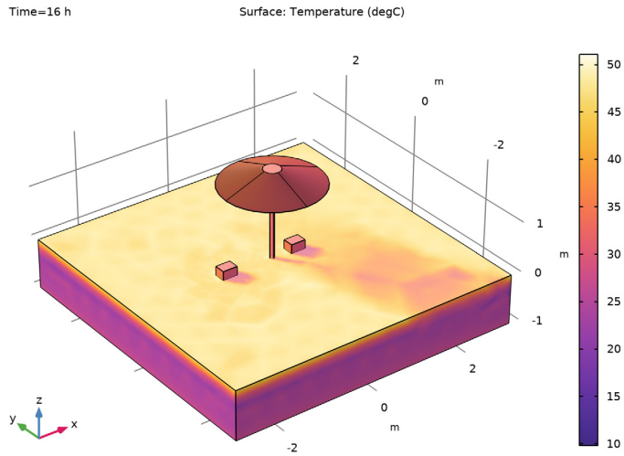
Figure 2: Temperature distribution.
