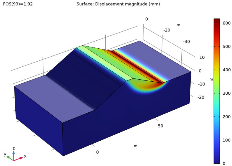
Figure 5: Displacement magnitude of the embankment dam just before the collapse of the slope.
