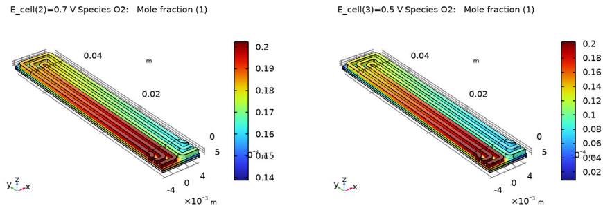
Figure 4: Oxygen mole fraction at 0.7 V (left) and 0.5 V (right).
