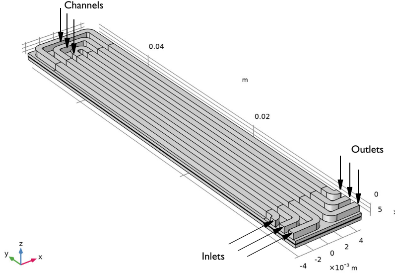
Figure 1: Model geometry.
