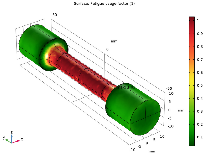
Figure 5: Fatigue usage factor Matake criterion.
