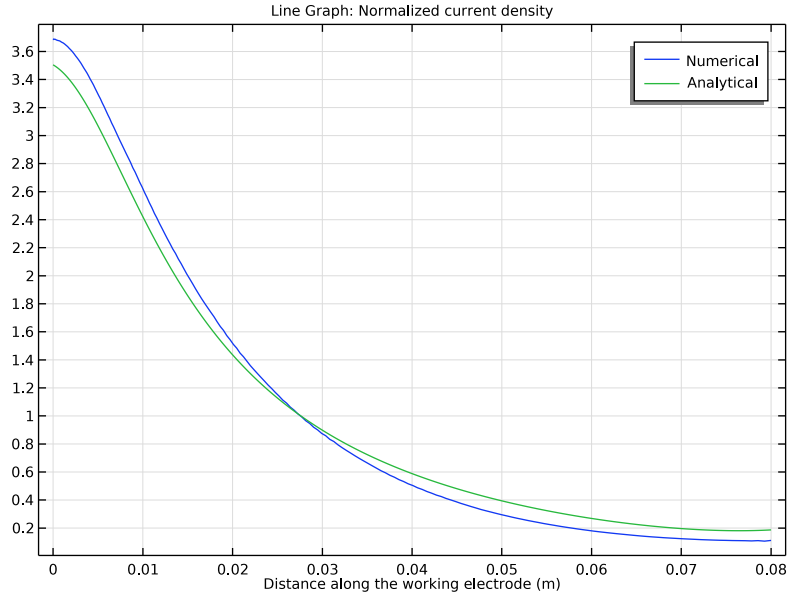
Figure 2: Normalized primary current density distribution obtained from the numerical model and the analytical expression.
