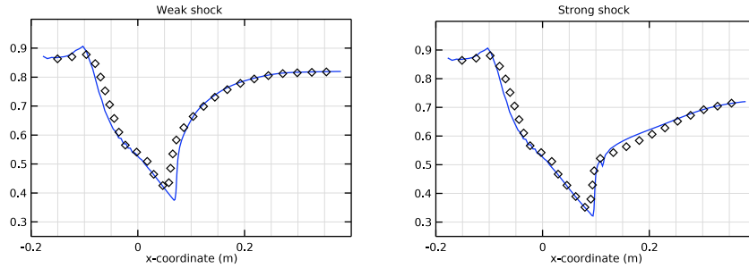
Figure 4: Top wall static pressure normalized by the inlet total pressure. Model results (lines) and experimental results (diamonds) are shown.
