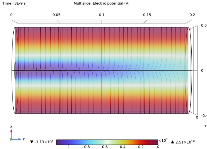
Figure 2: Electric potential in the relativistic beam. The magnitude of the potential is greatest at the beam waist.
