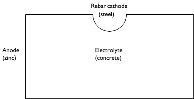
Figure 4: Model geometry. One electrolyte domain and two electrode surfaces.
