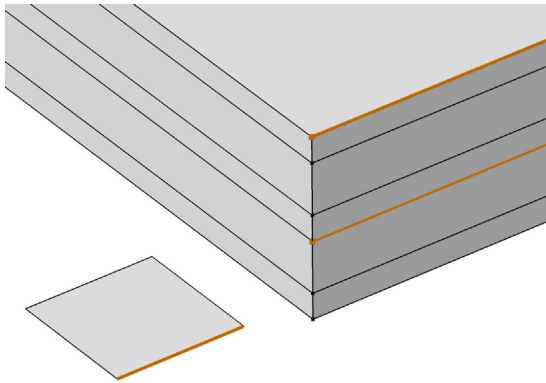
Figure 3-21: Edge selection with interfaces 'layer 2 - layer 3' and 'layer 5 up' selected.
