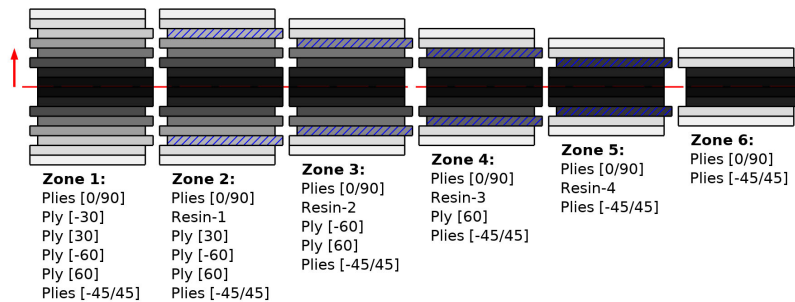
Figure 3-14: Zones created in the ply-based modeling approach. The layup in each zone can also be seen. A ply having sectioning represents the variable thickness ply.
