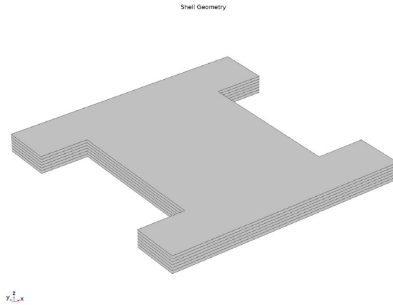
Figure 3-15: 3D solid geometric representation (scaled in thickness direction) of a composite laminate having six layers.
