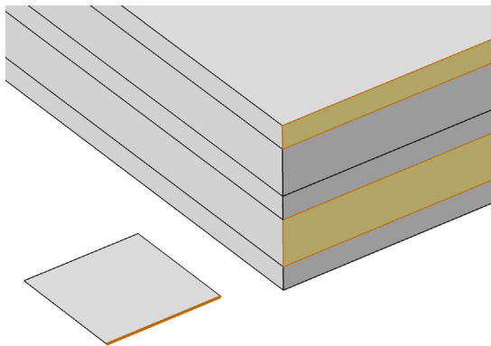
Figure 3-18: Edge selection with layers 2 and 5 selected.
