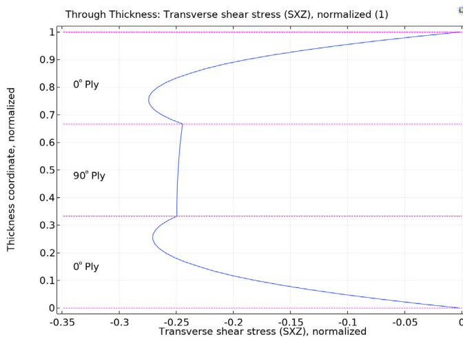
Figure 3-25: Example of a Through Thickness plot, where the transverse shear stress is plotted at a particular point on a composite laminate with three layers ([0/90/0]).
