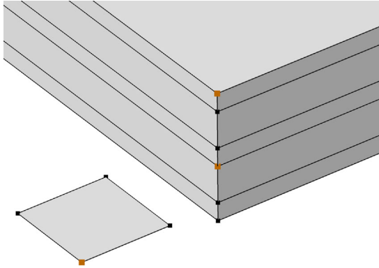
Figure 3-22: Point selection with interfaces 'layer 2 - layer 3' and 'layer 5 up' selected.
