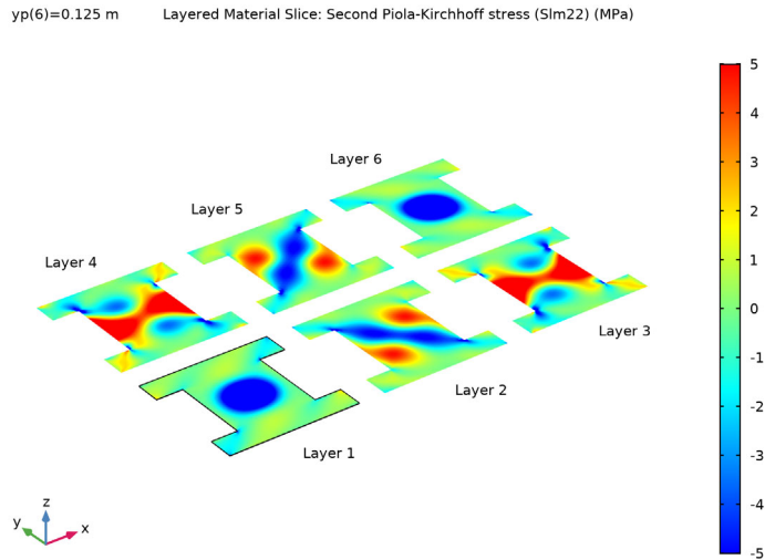
Figure 3-24: Example of a Layered Material Slice plot, where the Second Piola-Kirchhoff stress is plotted in all the layers of a laminate with six layers ([30/-45/75/-75/45/30]).
