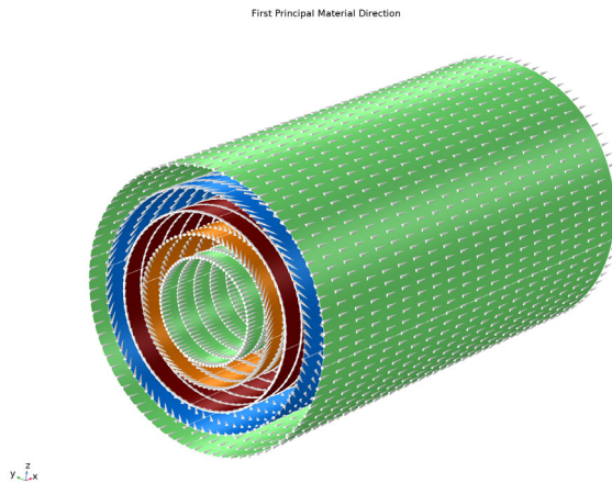
Figure 3-16: First principal material direction showing the fiber draping direction in each layer of a composite cylinder.
