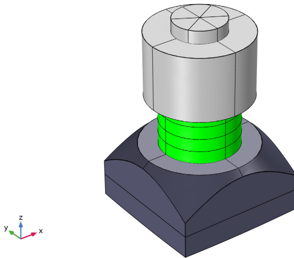
Figure 1: A tonpilz transducer. The aluminum head mass is shown in dark gray, the central steel bolt and steel tail mass are shown in light gray and the piezostack actuator with four disks of PZT-4 is shown in green.
