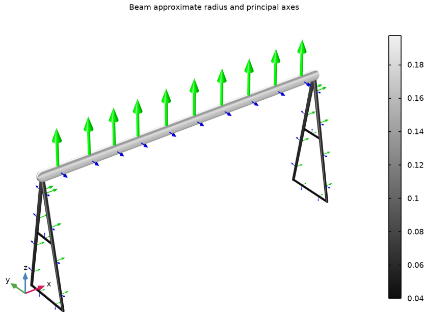
Figure 2: A sketch of the crane, with the stiffness of the members indicated (using size, grayscale, and arrows in the principal directions).
