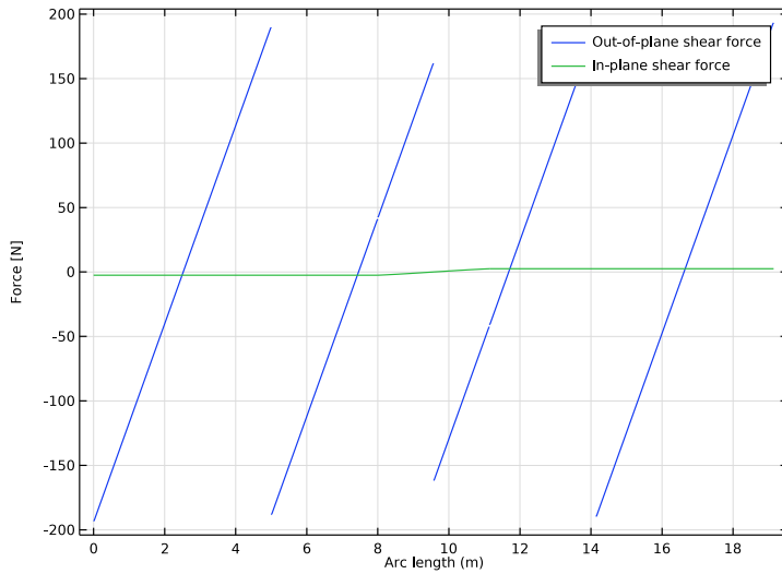
Figure 6: Shear forces.
