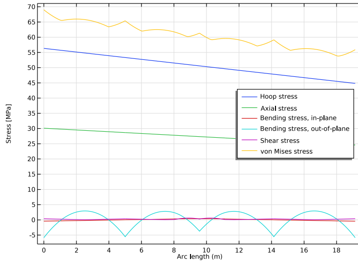
Figure 7: Stress contributions.
