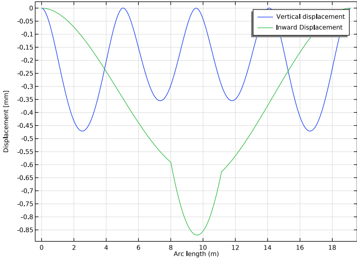
Figure 4: Pipe displacement.
