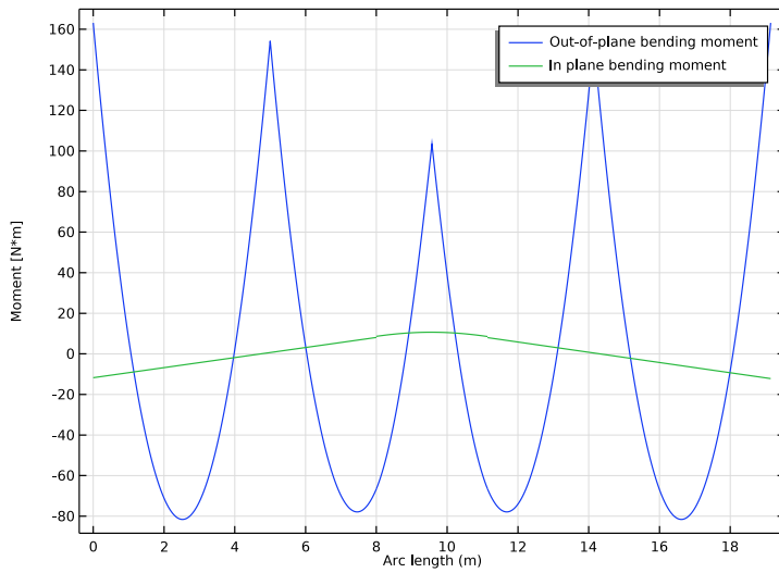
Figure 5: Bending moments.
