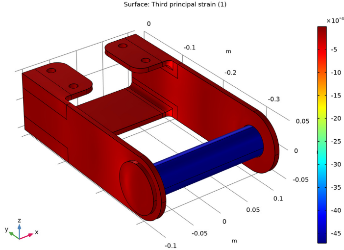
Figure 3: Strain distribution in the bracket.
