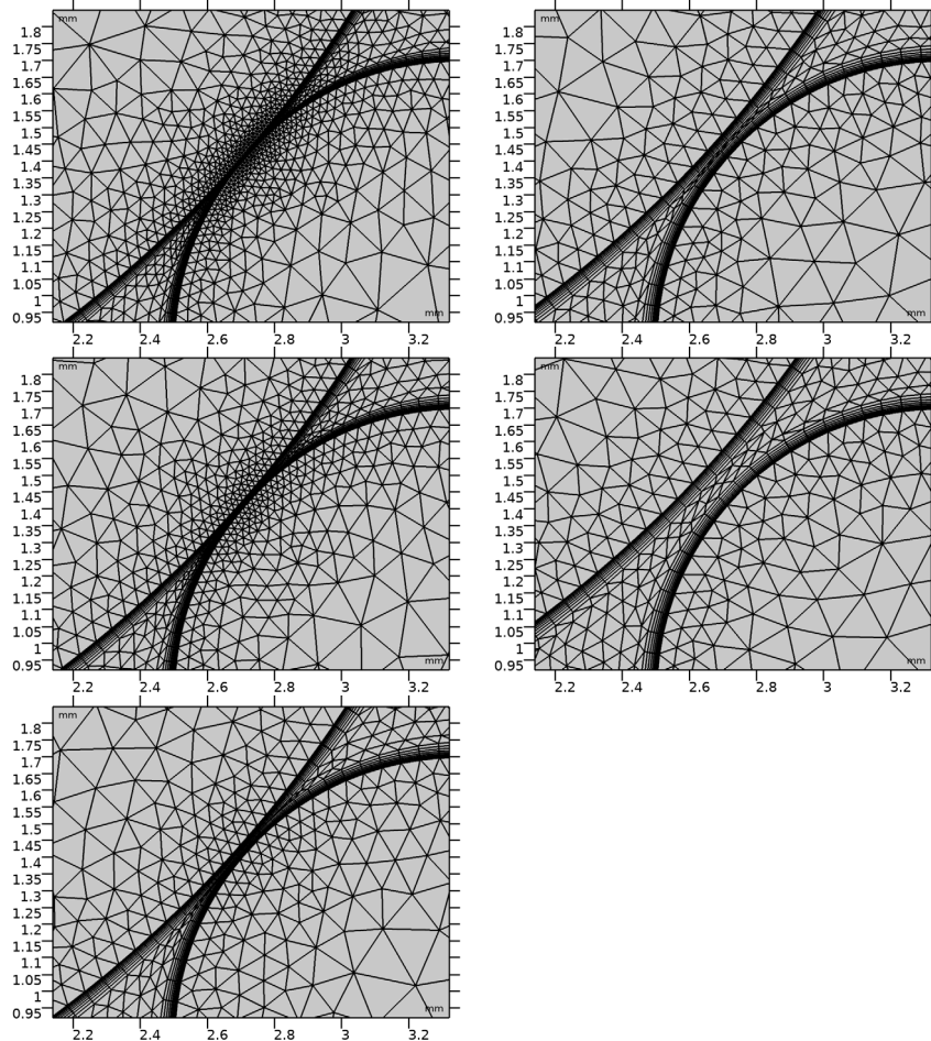
Figure 11: Mesh cases used during the computation (from top to bottom, left to right).
