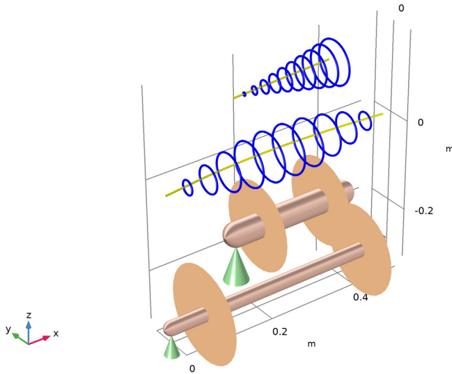
Figure 2: Whirl plot for the first mode.
