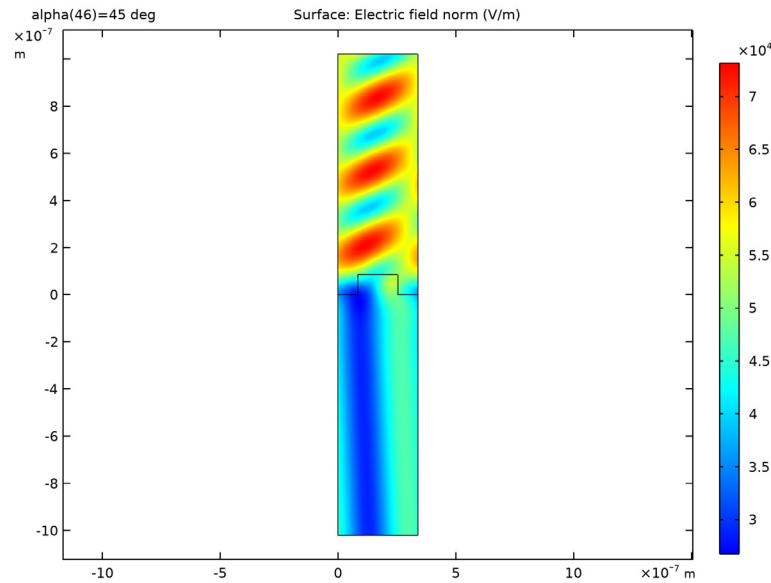
Figure 2: Norm of the electric field for a TE wave with an angle of incidence of 45 degrees.
