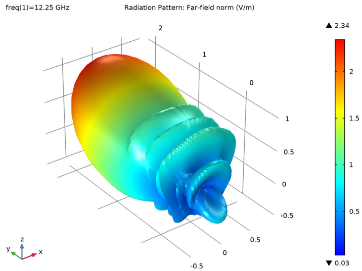
Figure 4: The 3D far-field radiation pattern is tilted toward the positive y -axis.
