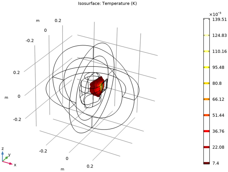
This is the isosurface plot of temperature.
