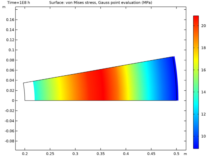
Figure 3: Distribution of von Mises equivalent stress at t = 10^8 h.
