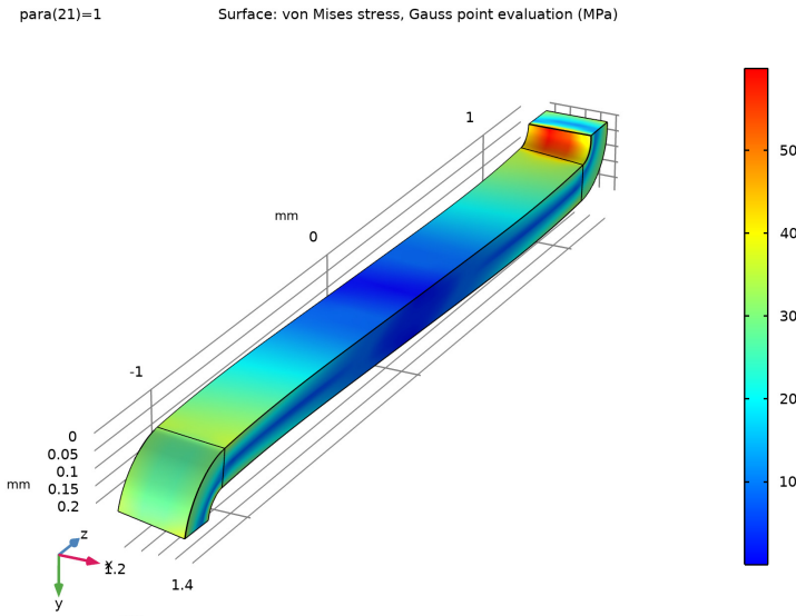
Figure 3: Stress and transformation state of one arm of the stent after crimping.
