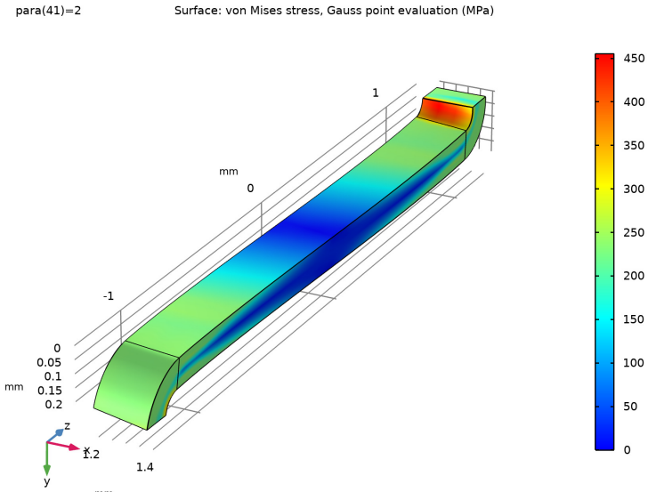
Figure 4: Stress and transformation state of one arm of the stent in the human body.
