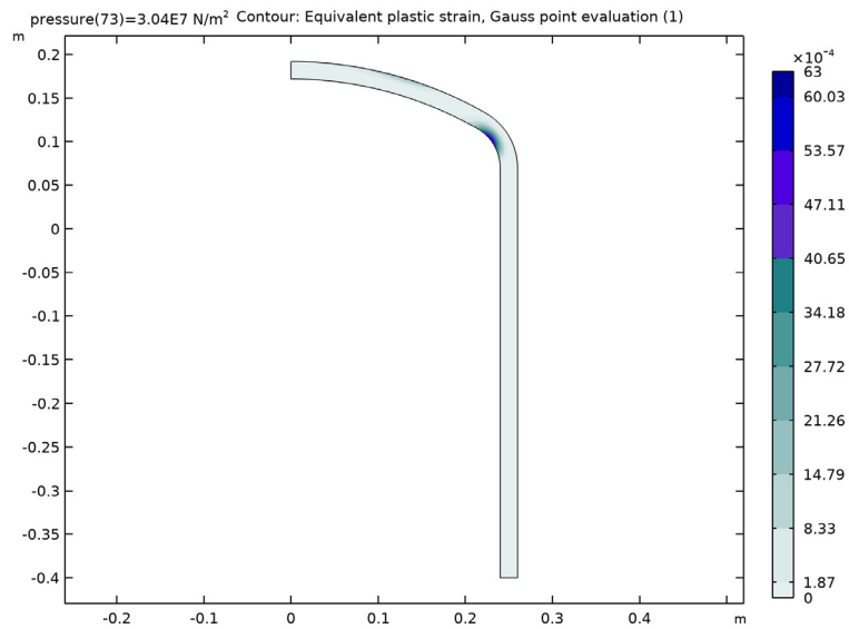
Figure 4: Equivalent plastic strain at 10% yielded volume.
