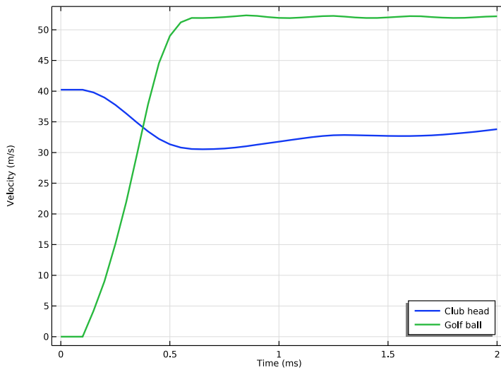
Figure 4: Average magnitude of the velocity in the club head and the golf ball.
