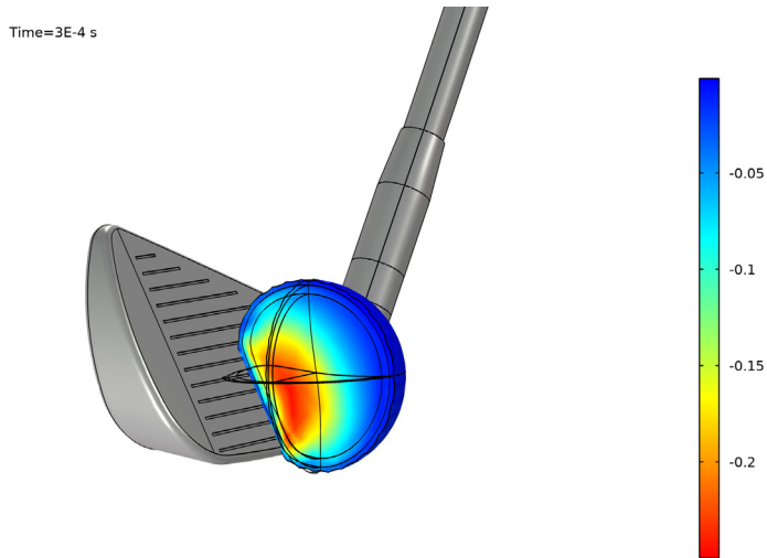
Figure 3: Deformation of the golf ball and distribution of the third principal (compressive) strain in the interior part of the ball at 0.3 ms.
