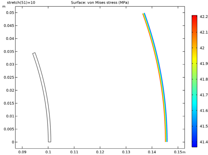
Figure 5: Distribution of von Mises stress on the modeled 2D cross section for the neo-Hookean material at maximum inflation.
