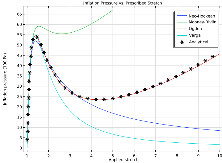
Figure 3: Computed inflation pressure as a function of circumferential stretch for different material models, compared to the analytical expression for the Ogden material model.
