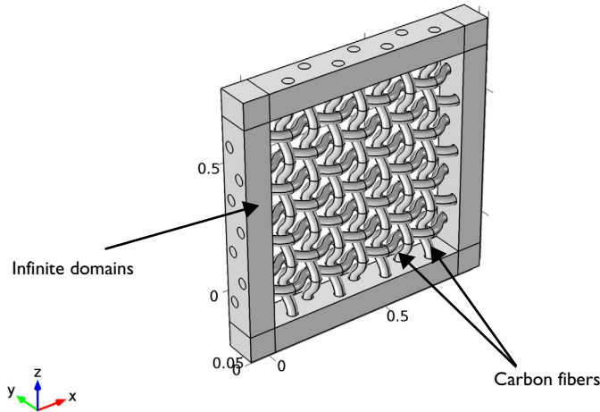
Figure 1: Model geometry: fibers embedded in an epoxy matrix (hidden) with infinite element domain.
