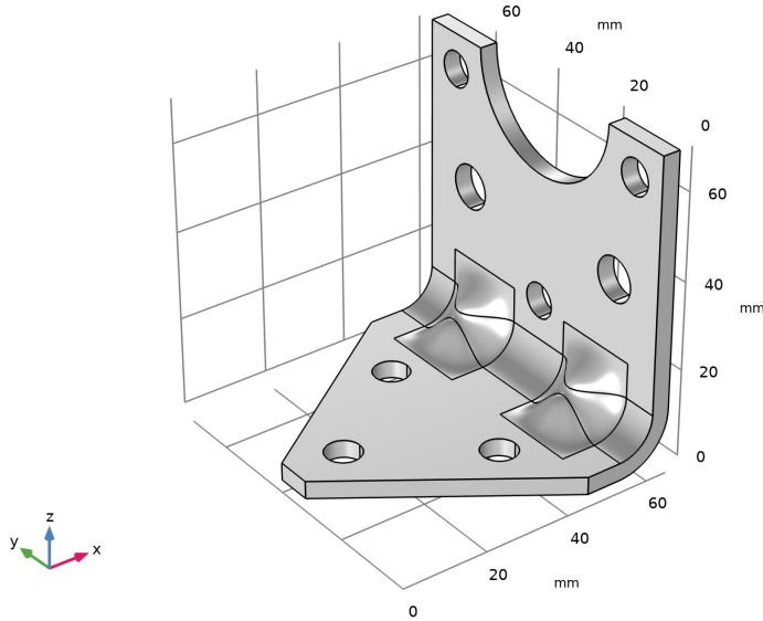
Figure 4: Initial geometry.
