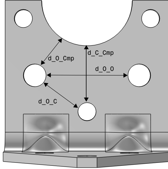
Figure 3: Geometrical constraints.
