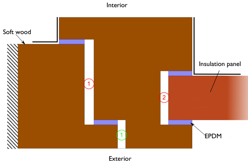
Figure 3: Geometry of the wood frame with an insulation panel.
