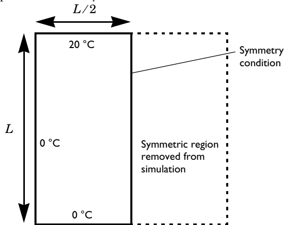
Figure 1: Geometry and boundary conditions of ISO 10211:2007 test case 1.
