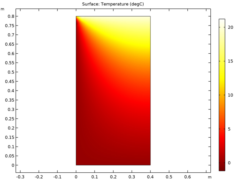
Figure 3: Temperature distribution of ISO 10211:2007 test case 1.
